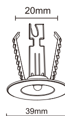
LED Holder
